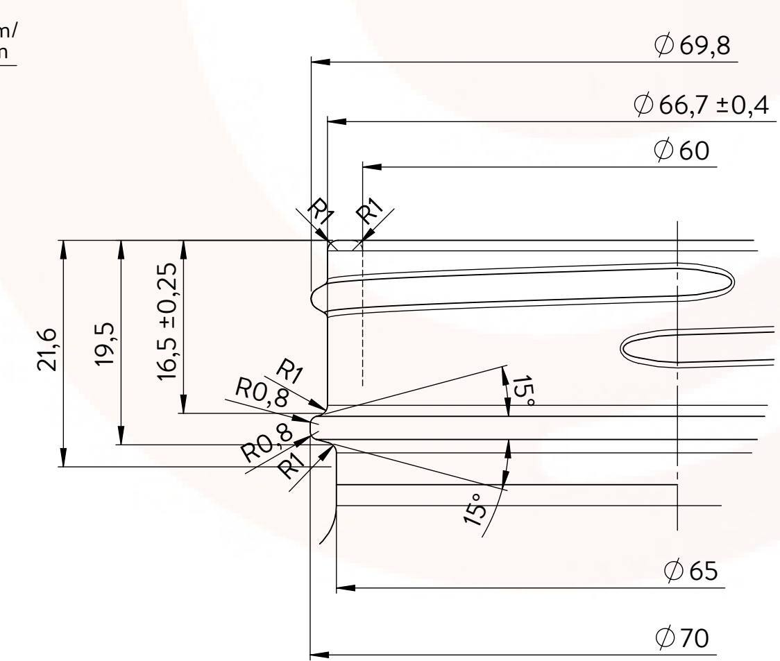
DETALLE A Boca GPI-450-70 DETAIL A Neck GPI-450-70 ESCALA 2 : 1
